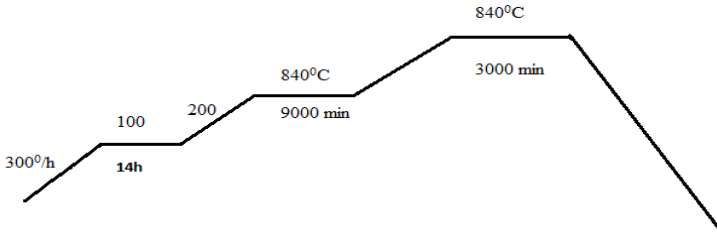
Figure 2. Schematic representation of heat treatment
