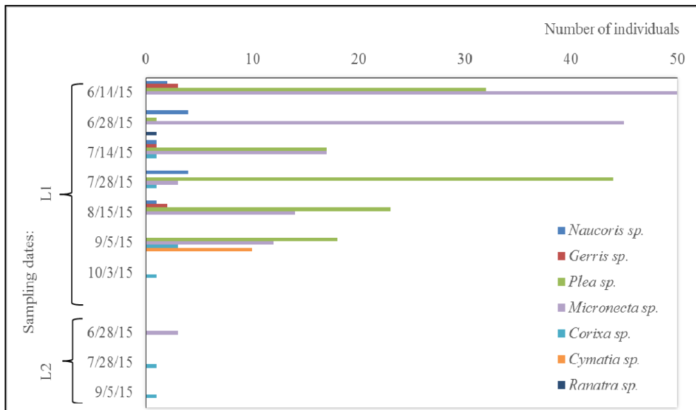
Figure 6. Number of individuals belonging to different Hemiptera (Heteroptera) individuals from Lake Sucutardul Mare ( L1 ) and its temporary fry pond ( L2 ) (see text for sampling date abbreviations)
