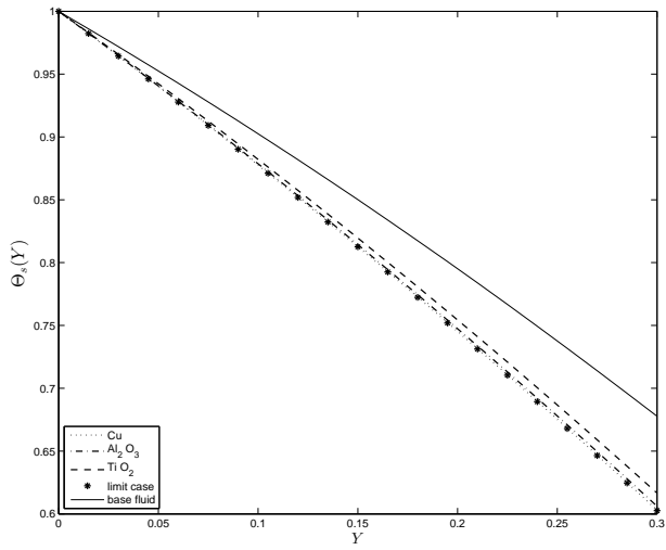
FIGURE 2. Solid temperature
