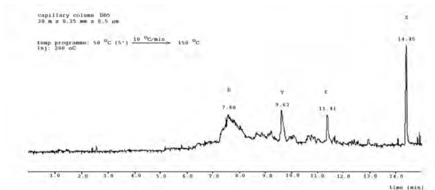
Fig. 1. Analytes (BTEX) collected on the SPME fiber, and separated on the DB-5 capillary column
