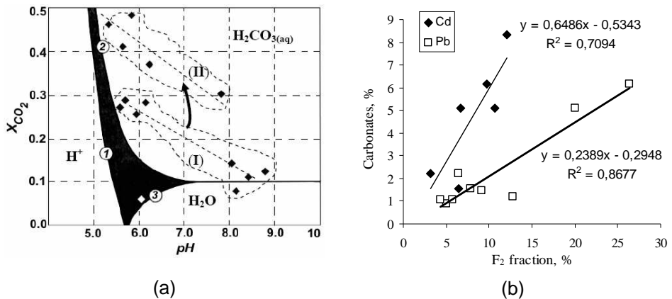
Fig. 1. (a) The possible mechanisms of calcite dissolving in antropoc soils in function of pH and P_{CO_2} (estimated from [CO_3^{2-}] solubilized, at 25°C) [11]. Lines (1), (2) and (3) delimited the domains in which [H^+] , [H_2O] and [H_2CO_{3(aq)}] control the kinetics of calcite dissolving processes. On diagram are demarked the evolution tendency of global calcite dissolving processes at increasing of Cd and Pb concentration from studied antropoc soils: (I) calcite dissolving is control by pH, (II) calcite dissolving is control by [H_2CO_{3(aq)}] . (b) The correlations between the weights (% from total content) of Cd and Pb F2 fractions (bonded on carbonates minerals) and total carbonates content from antropoc soil samples.
