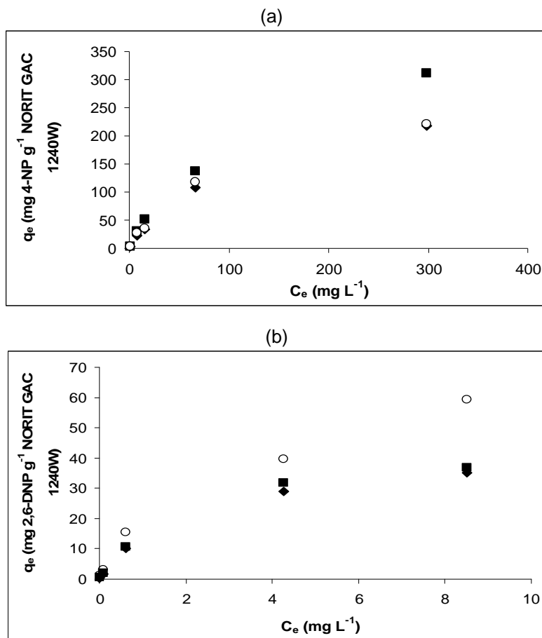
Figure 1. The fit of experimental data ( \blacklozenge ) to Langmuir ( \blacksquare ) and Freundlich ( \circ ) models at 25^\circ\text{C} for: (a) 4-nitrophenol and (b) 2, 6-dinitrophenol in water.
