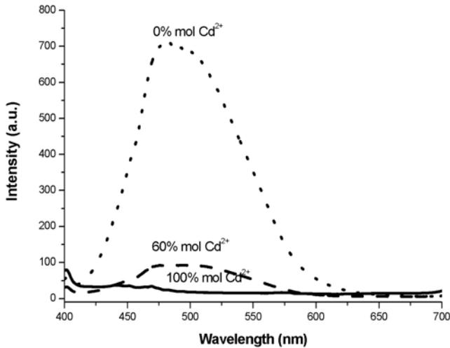
Figure 7. Emission spectra of ZnCdS:Cu films obtained from chemical bath with different Cd 2+ amounts
