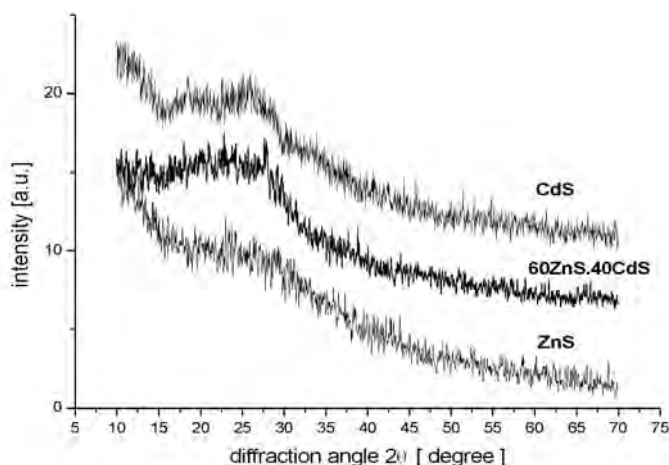
Figure 6. X-ray scattering curves of some ZnCdS films (MoK α )
