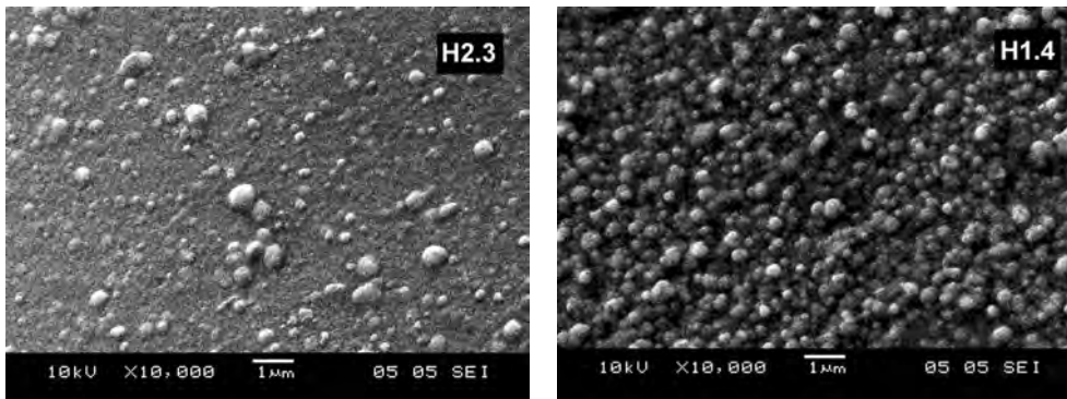
Figure 5. SEM images of ZnS film (H2.3) and CdS film (H1.4)
