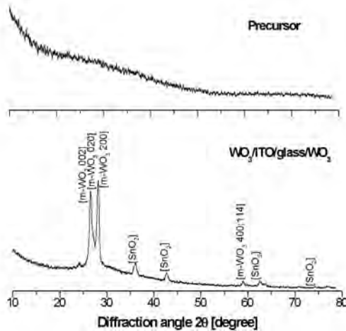
Figure 6. XRD patterns for PTA precursor and the corresponding heterostructure WO 3 /ITO/Glass/WO 3 (film R415).
