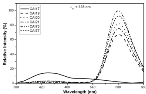
Figure 3. Emission spectra of \text{ZnS}:\text{Mn}^{2+} powders obtained from acetate mixtures with various \text{Mn}^{2+} concentration.
