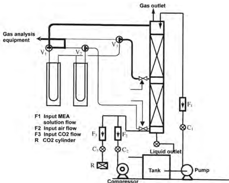
Figure 1. Gas – liquid packed absorption column
