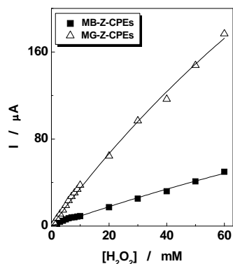
Figure 5. Calibration curves for \text{H}_2\text{O}_2 at MB-Z-CPEs and MG-Z-CPEs. Experimental conditions: applied potential, -400 mV vs. \text{Ag}|\text{AgCl}/\text{KCl}_{\text{sat}} ; supporting electrolyte, 0.1 \text{ M} phosphate buffer, pH 6.0.
