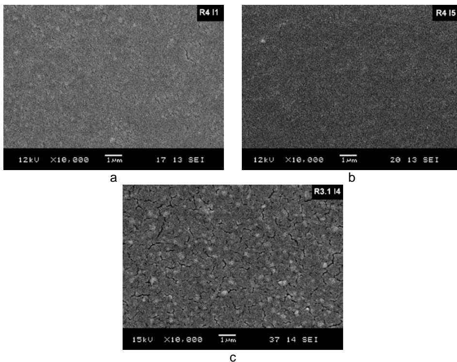
Figure 7. SEM images of WO 3 film surface: (a) one layer (350°C) (b) five layers (350°C) and (c) one layer (550°C).
