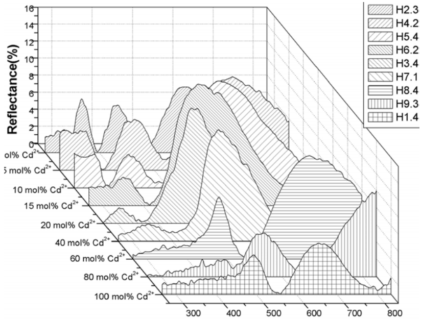
Figure 4. Specular reflectance spectra of ZnCdS thin films obtained from chemical bath with different Cd 2+ amounts
