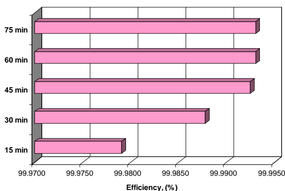
Figure 9. Removal efficiency evolution in time during lead removal process on Orașul Nou bentonite sample in dynamic regime (3D shaker), C i = 54 mg Pb 2+ /L, 2 g bentonite, 20 ml solution.
