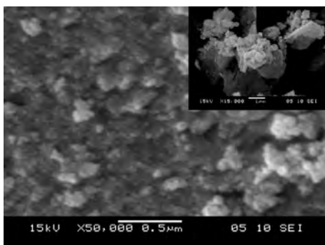
Figure 5. SEM image of ZnS:Mn 2+ sample (inset scale bar = 1 \mu\text{m} )
