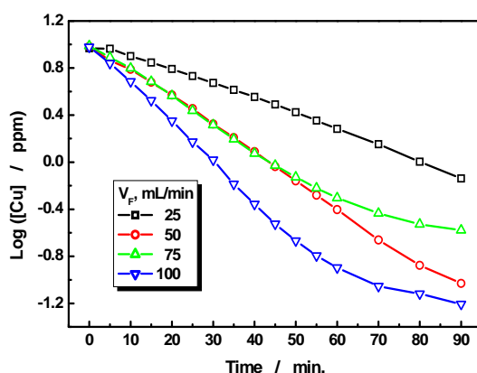
Figure 2. The evolution in time of the copper concentration for different volume flow rate (ε W.E. = -200 mV/RE; 7.5 mM Na 2 SO 4 )
