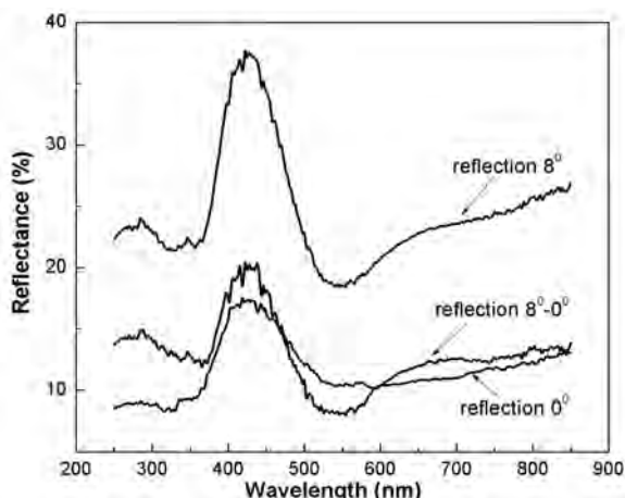
Figure 4. Reflectance spectra for the multilayer WO_3 film (R415) measured on ITO face.
