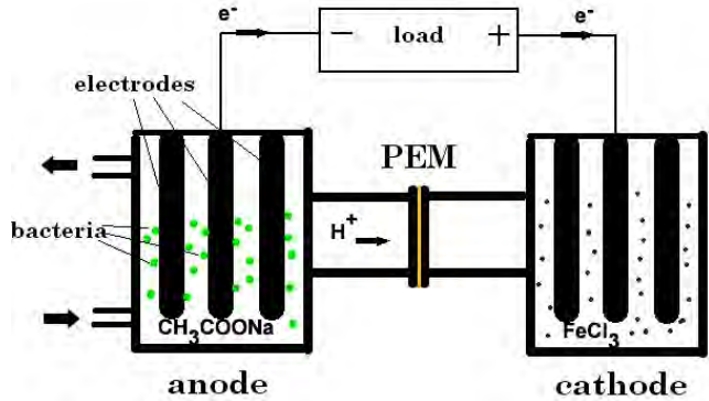
Figure 1. Biobattery representation
