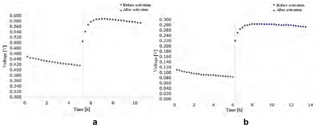
Figure 2. Voltage-time dependency.
