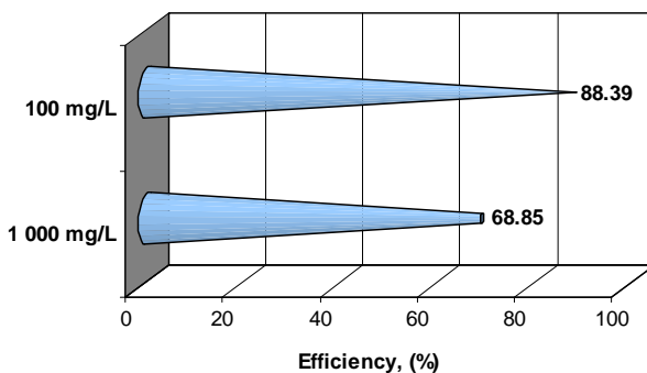
Figure 6. Phenol initial concentration influence over the overall efficiencies in the phenol CWAO process, at constant air flow and constant temperature, 60 L/h, 80°C, for \text{Fe}^{(3+)} -DCA catalyst (0.1 g catalyst).
