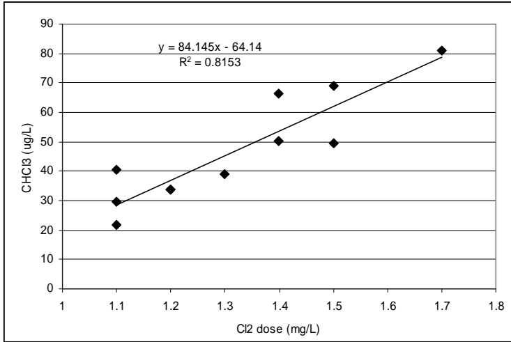
Figure 1. Chlorine dose as function of CHCl 3 concentration in Gilau WTP
