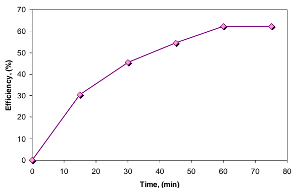
Figure 10. Removal efficiency evolution in time during cadmium removal process on Orașul Nou bentonite sample in dynamic regime (3D shaker), C i = 25 mg Cd 2+ /L, 2 g bentonite, 20 ml solution.
