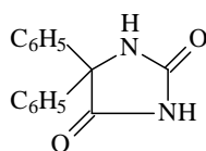
Figure 1. Molecular structure of phenytoin
