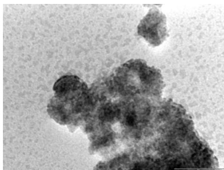
Figure 6. TEM image of ZnS:Mn 2+ (scale bar=50 nm)
