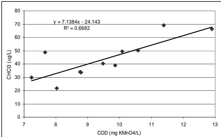
Figure 2. Relationship between CHCl 3 (ug/L) and presence of natural organic mater in water
