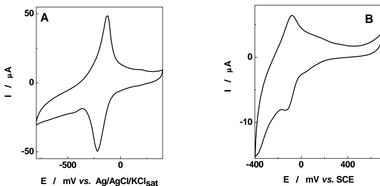
Figure 1. Cyclic voltammograms for MB-13X-CPEs (A) and MG-13X-CPEs (B). Experimental conditions: starting potential, -650 mV vs. Ag|AgCl/KCl sat (A) and -400 mV vs. SCE (B); potential scan rate, 10 mV s -1 ; supporting electrolyte, 0.1 M phosphate buffer, pH 7.
