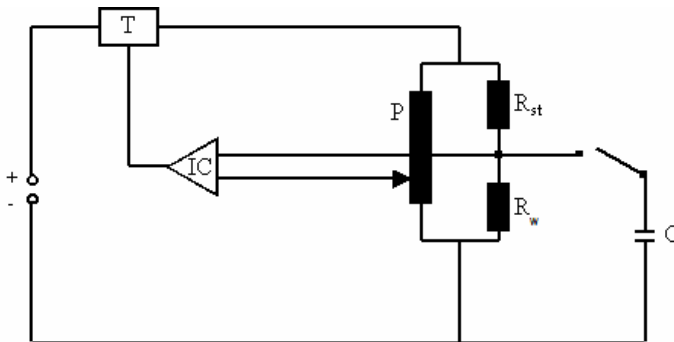
Figure 4. Schematic representation of the electrical circuit able to heat the platinum wire according to a quasi-rectangular profile
