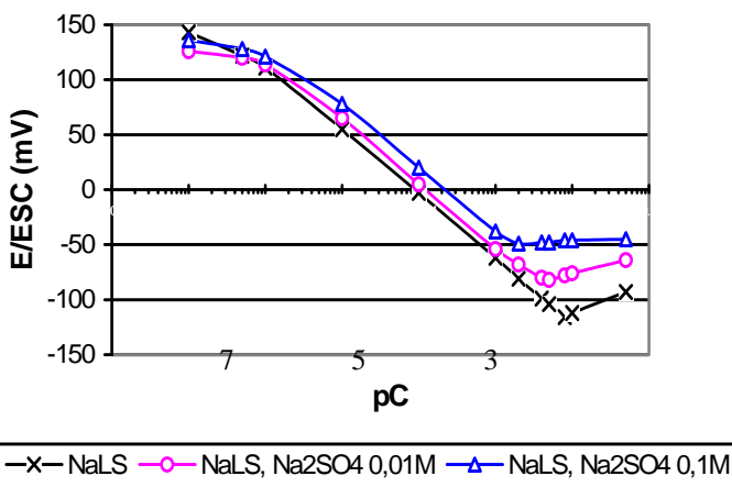
Figure 1. The influence of the ionic strength on the response functions of the laurylsulphate sensible electrode: X - pure NaLS solutions; O - NaLS solutions with Na 2 SO 4 0.01 M (J=0.03) Δ- NaLS solutions with Na 2 SO 4 0.1 M (J=0.3)
