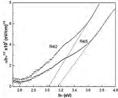
Figure 5. Plot of (\alpha h\nu)^{1/2} vs h\nu for WO 3 films.
