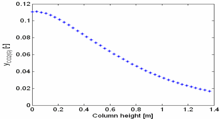
Figure 2. CO 2 concentration (in gas phase) along the column height
