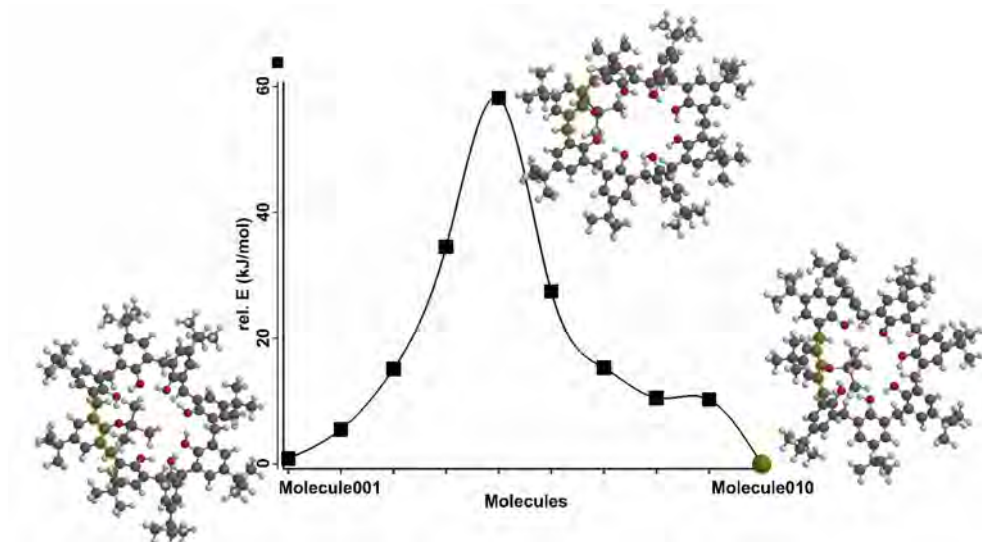
Figure 1. A plot of the PM3 calculated energies against the HC...CH (marked) dihedral angle for the monosubstituted calix[8]arene.
