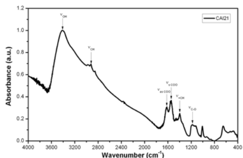
Figure 2. FT-IR spectrum of ZnS:Mn 2+ sample (CAI21)
