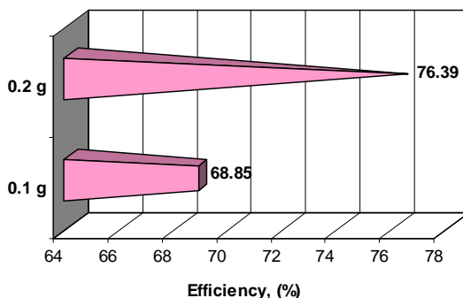
Figure 5. Catalyst quantity influence over the maximum overall efficiencies obtained in the phenol CWAO process, at constant air flow and constant temperature, 60 L/h, 80°C, for \text{Fe}^{(3+)} -DCA catalyst ( C_i = 1000 \text{ mg phenol/dm}^3 ).
