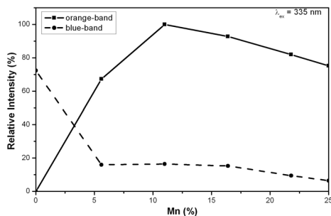
Figure 4. Relative intensity of the orange and blue bands versus Mn concentration (blue band is 5 times multiplied)
