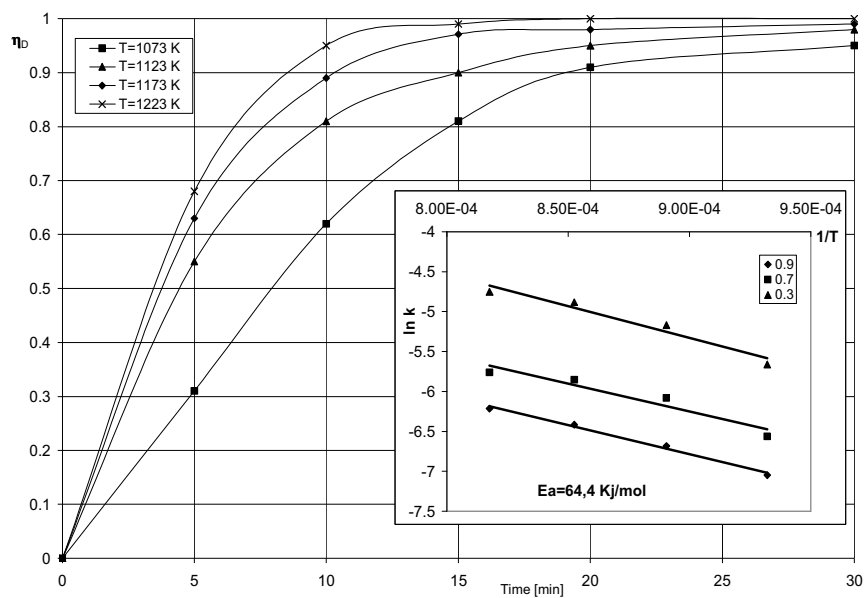
Fig. 3. Temperature influence over the decomposition degree of PCC granules with d_p=0.063\text{mm} .
