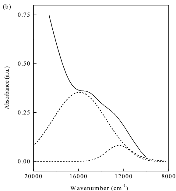
Figure 4. Vis-NIR absorption spectrum of \text{Bi}_2\text{W}_{20}\text{V}^{\text{IV}}_2 in aqueous solution ( c = 10^{-4} \text{ mol dm}^{-3} ). The Gaussian components are shown with dashed lines.
