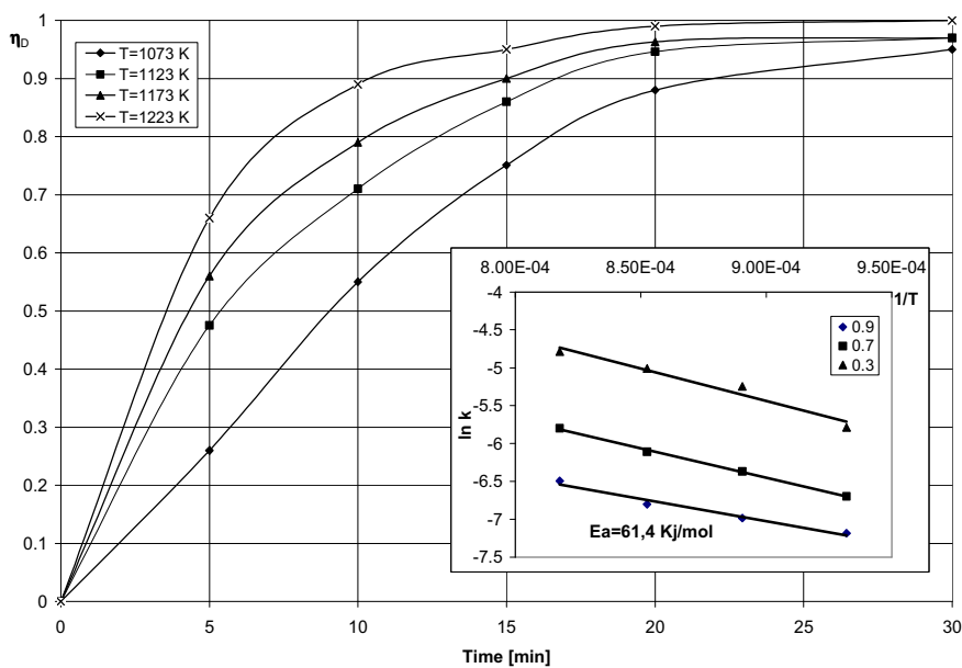
Fig. 4. Temperature influence over the decomposition degree of PCC granules with d_p=0.18\text{mm} .
