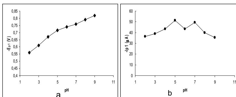
Figure 3. The variation of: (a) the first reduction peak potential ( E_{p1} ); (b) current intensity, with the pH, for a 4.5 \times 10^{-4} \text{ M} 2,6-DNP solution in Britton-Robinson buffer at different pH values WE: GC; RE: Ag/AgCl,KCl; CE: Pt; v : 50\text{mV s}^{-1} ; s : 10 \mu\text{A V}^{-1} .
