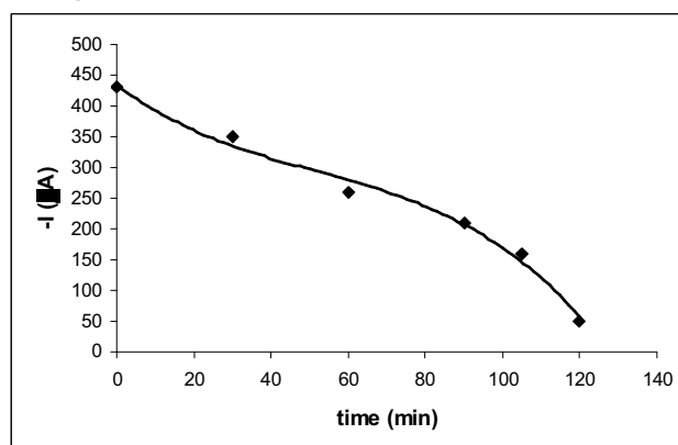
Figure 6. The variation of the reduction peak intensity during electrochemical reduction process for 10^{-2} M 4-NP in 0.2 N H_2SO_4 , on graphite cathode (experimental set-up B); i: 20 mA cm^{-2} .
