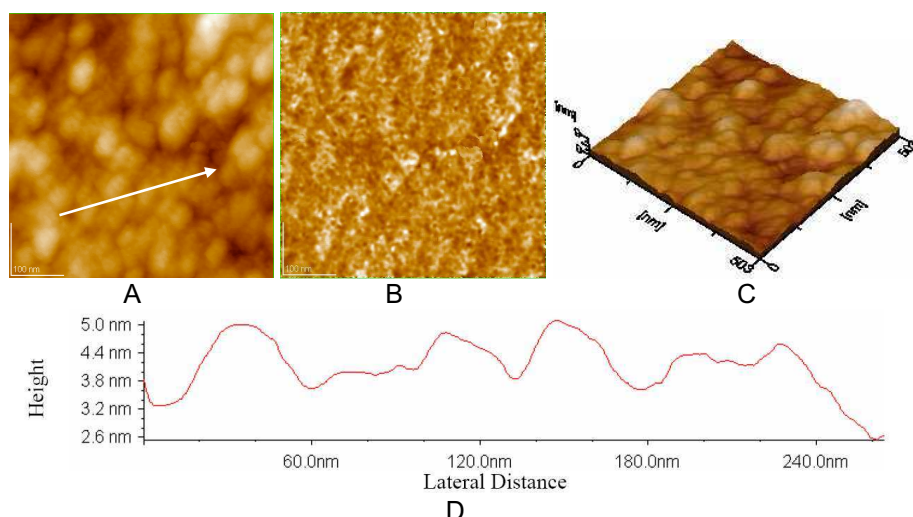
Fig. 2. Collagen film on glass, zone 1: A) 2D – topography B) phase image C) 3D-topography, D) profile of the cross section along the arrow in Fig. 2A. Scanned area: 0.5 \mu\text{m} x 0.5 \mu\text{m} .
