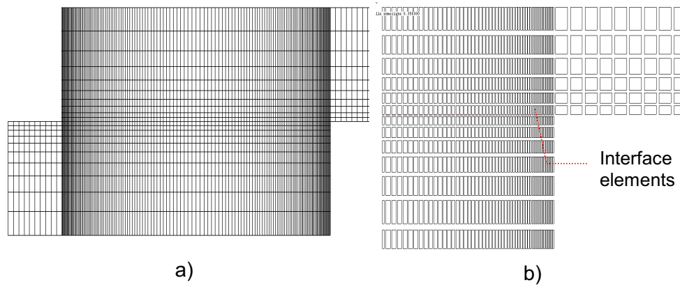
Figure 3. Numerical modeling of a double-lap bonded joint with interface elements: a) assembly; b) detail.
