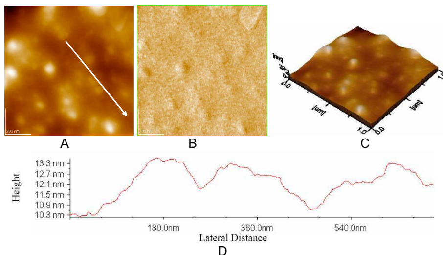
Fig. 6. Doxorubicin film on glass: A) 2D – topography; B) phase image; C) 3D-topography; D) profile of the cross section along the arrow in Fig. 6A. Scanned area: 1\ \mu\text{m} \times 1\ \mu\text{m} .
