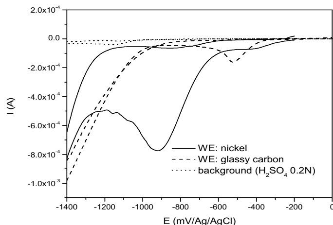
Figure 2. Cyclic voltammograms for a ( 10^{-2} \text{ M} ) 4-NP solution in 0.2\text{N H}_2\text{SO}_4 WE: GC and Ni; RE: Ag/AgCl,KCl; CE: Pt; v : 50\text{mV s}^{-1} ; s : 100 \mu\text{A V}^{-1} .
