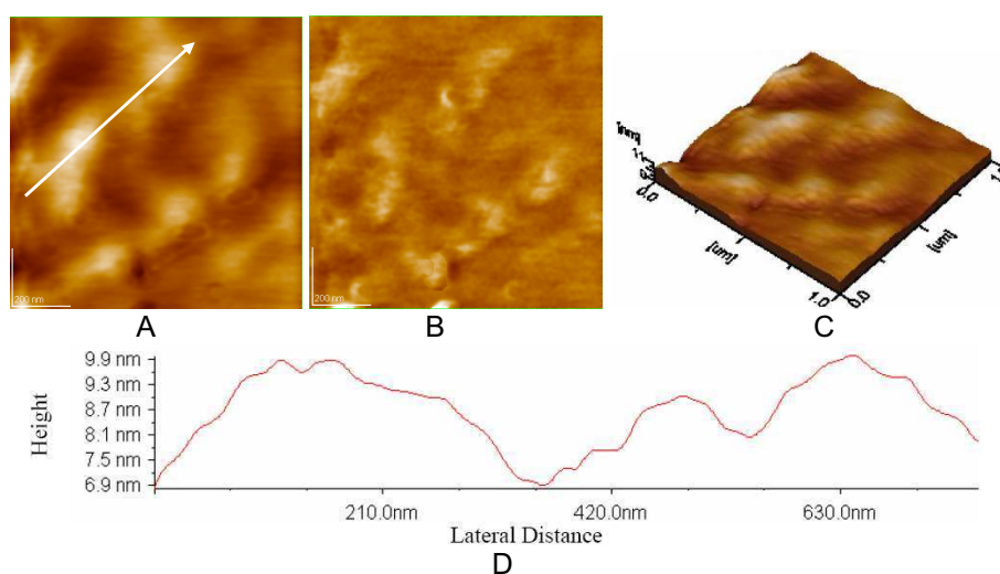
Fig. 7. Lipoic acid film on glass: A) 2D – topography; B) phase image; C) 3D-topography; D) profile of the cross section along the arrow in Fig. 7A. Scanned area: 1\ \mu\text{m} \times 1\ \mu\text{m} .
