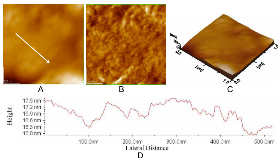
Fig. 3. Collagen film on glass, zone 2: A) 2D – topography B) phase image C) 3D-topography, D) profile of the cross section along the arrow in Fig. 3A. Scanned area: 1 \mu\text{m} x 1 \mu\text{m} .
