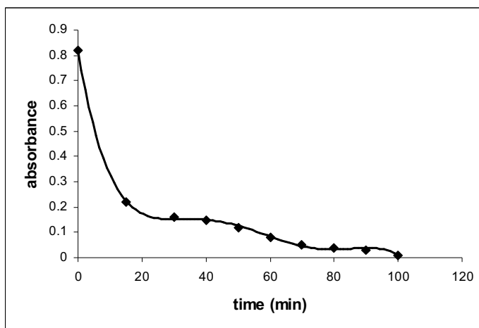
Figure 8. Spectrophotometric control of electrochemical reduction process for 4.5 \times 10^{-5} M 2,6-DNP in (0.1N) NaCl, on graphite cathode (experimental set-up C). \lambda_{\max} = 440 nm; \log \epsilon = 3.58 .
