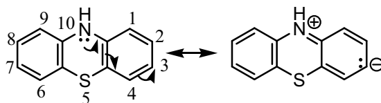
Figure 1. Phenothiazine: IUPAC numbering and resonance structures.
