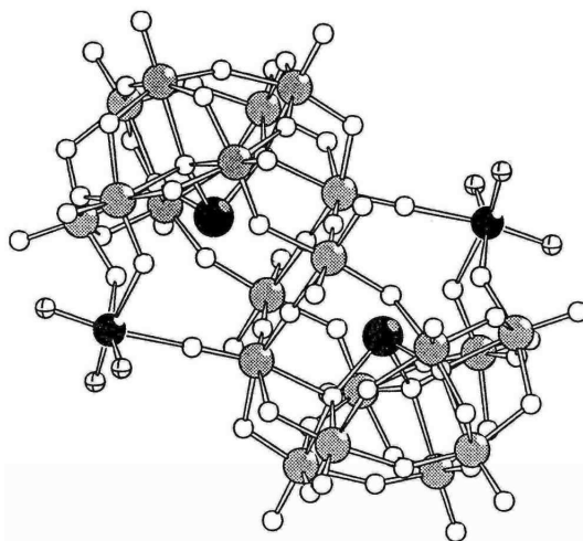
Figure 1. Ball-and-stick representation of the mixed addenda [X_2W_{20}M^{(n+)}_2O_{70}(H_2O)_6]^{(14-2n)-} polyoxometalate structure (X large dark spheres, W large gray spheres, M medium-sized dark spheres, O small white spheres, H_2O small white spheres with crossing lines).
