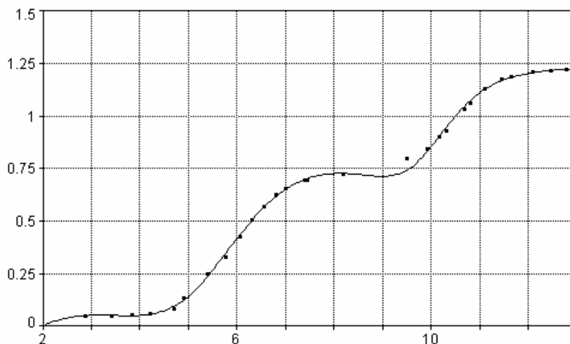
Figure 2. The plot absorbance at 490 nm vs. pH' corresponding to the spectra from Figure1
