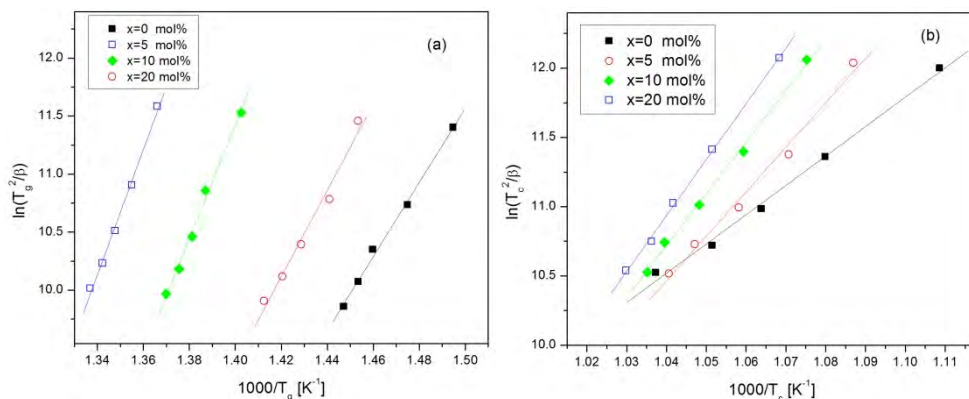
Figure 2a and 2b. The dependences \ln(T_g^2/\beta) on 10^3/T_g for the (\text{Fe}_2\text{O}_3)_x \cdot (\text{P}_2\text{O}_5)_{40} \cdot (\text{ZnO})_{(60-x)} glasses and the dependences \ln(T_c^2/\beta) on 10^3/T_c for the (\text{Fe}_2\text{O}_3)_x \cdot (\text{P}_2\text{O}_5)_{40} \cdot (\text{ZnO})_{(60-x)} glasses
