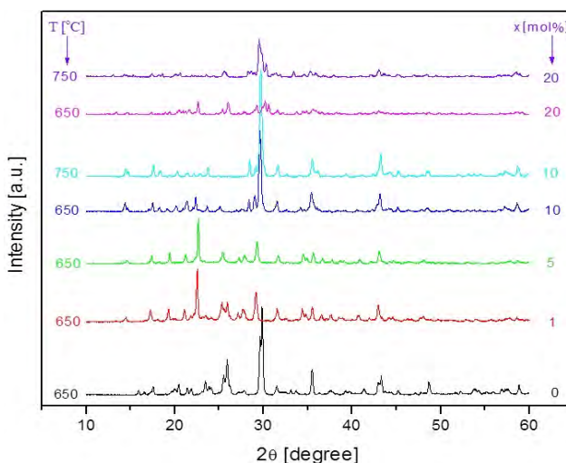
Figure 3. The XRD patterns of (\text{Fe}_2\text{O}_3)_x \cdot (\text{P}_2\text{O}_5)_{40} \cdot (\text{ZnO})_{(60-x)} glass ceramics
