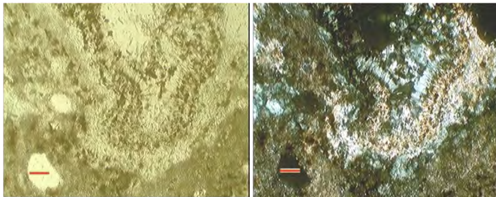
Figure 3. a (1N), b (N+) Sample 3, burned at 1220 °C: around the pore (top centre) was developed a ring with zonal structure: in the core - a radial lath - like alite ring overgrew by belite III with iron exsolutions and covered by belite I, the later being corroded by matrix phases (rough surface, due to reducing burning conditions). Scale bar 50 \mu m
