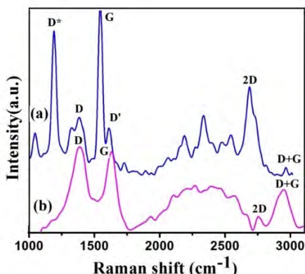
Figure 1. Raman spectra of the samples produced by pulsed laser ablation in (a) liquid nitrogen and (b) distilled water environments
