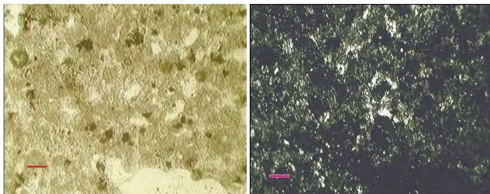
Figure 5. a (1N), b (N+). Sample 11A, burned at 1240°C: slightly differentiated interstitial material consists of yellowish green sulphoaluminate and ferrite; in the image centre there is a little pore with belite I ring overgrew by a belite II. Low cooling rate. Scale 50 \mu\text{m}
