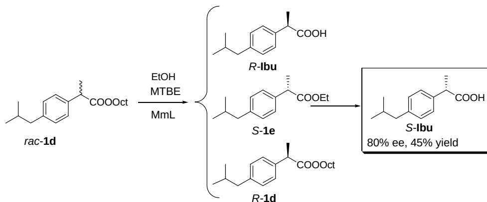
Scheme 3. Preparative scale synthesis of ( S )-Ibuprofen
