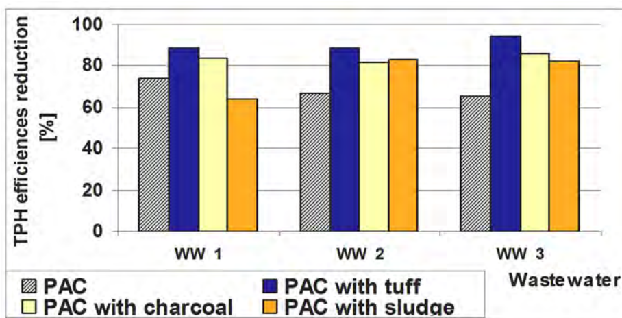
Figure 1. TPH reduction efficiency in WW 1- WW 3 samples treated with PAC coagulant agent used OD or RD in coagulation stage in absence/presence of coagulation aids.
