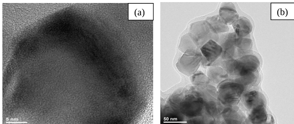
Figure 4. TEM images of the \text{CoFe}_2\text{O}_4 nanoparticles at a scale of 5 nm (a), and 50 nm (b)
