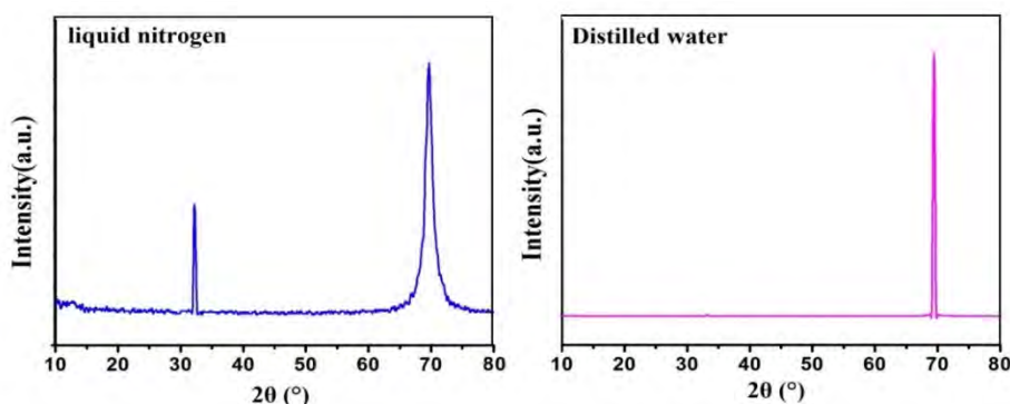
Figure 4. X-ray diffraction pattern of the samples produced by pulsed laser ablation
