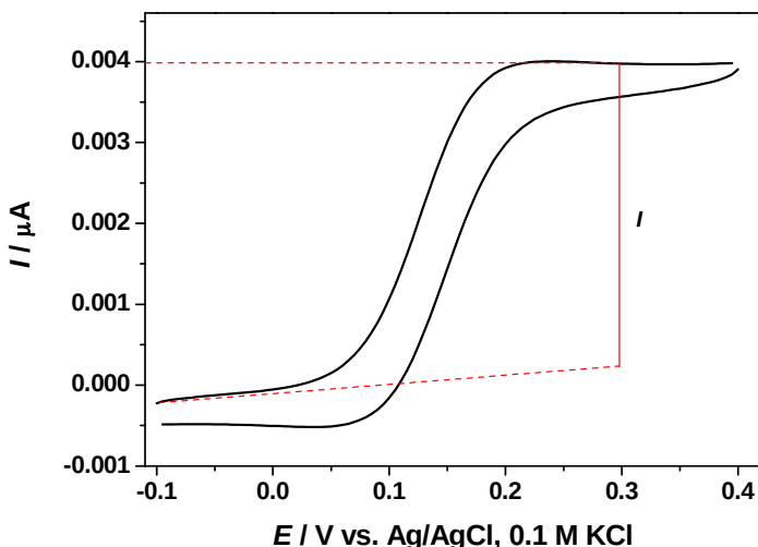
Figure 2. Representative CV recorded with a fabricated micro-electrochemical cell in 1 mM FcMeOH and 0.1 M KCl background electrolyte. Scan rate 0.05 \text{ Vs}^{-1} .
