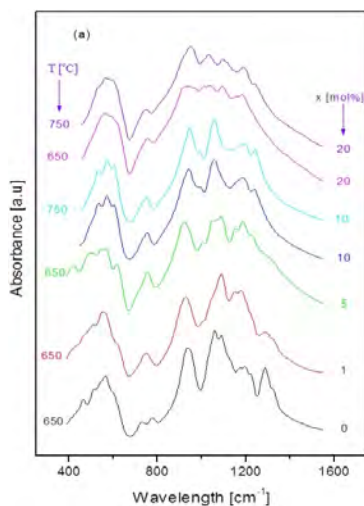
Figure 4. The FTIR spectra for the studied glass ceramics
