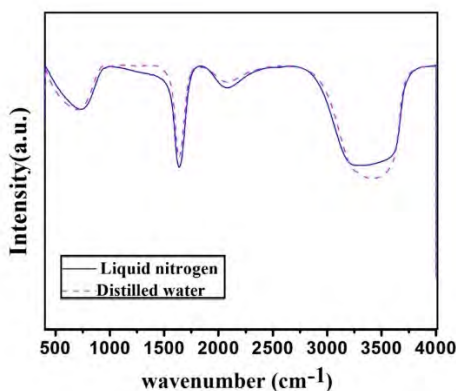
Figure 5. FTIR spectra of the samples
