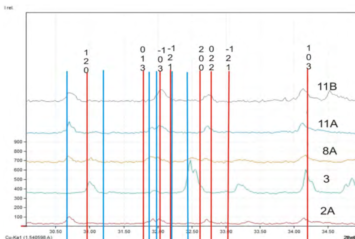
Figure 9. Detail of XRD patterns ( 2\theta = 30 - 35^\circ and reflections were recalculated for Cu-Kα1 for comparison with belite database) of samples 2A, 3, 8A, 11A, 11B. The reflexions of \alpha' -belite and \beta -belite were marked with different colors. The Miller indexes of \beta -belite crystallographic faces are indicated.
