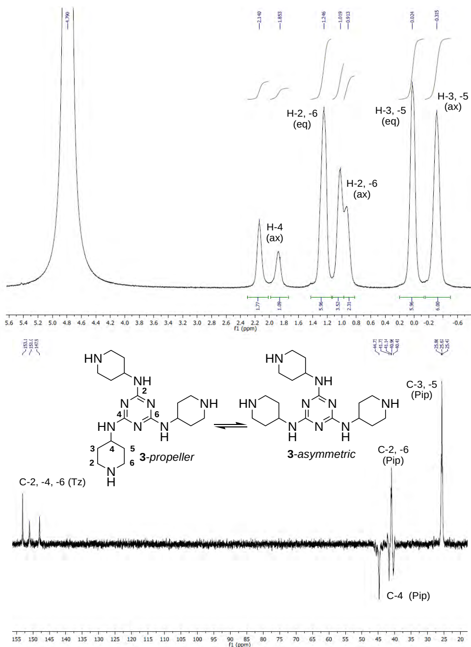
Figure 3. 1 H- and 13 C- J mod -NMR spectra (400 MHz, D 2 O+DCl, pH = 0.5-1, 298 K) of compound 3 . The protonated forms of 3 should be deduced implicitly.
