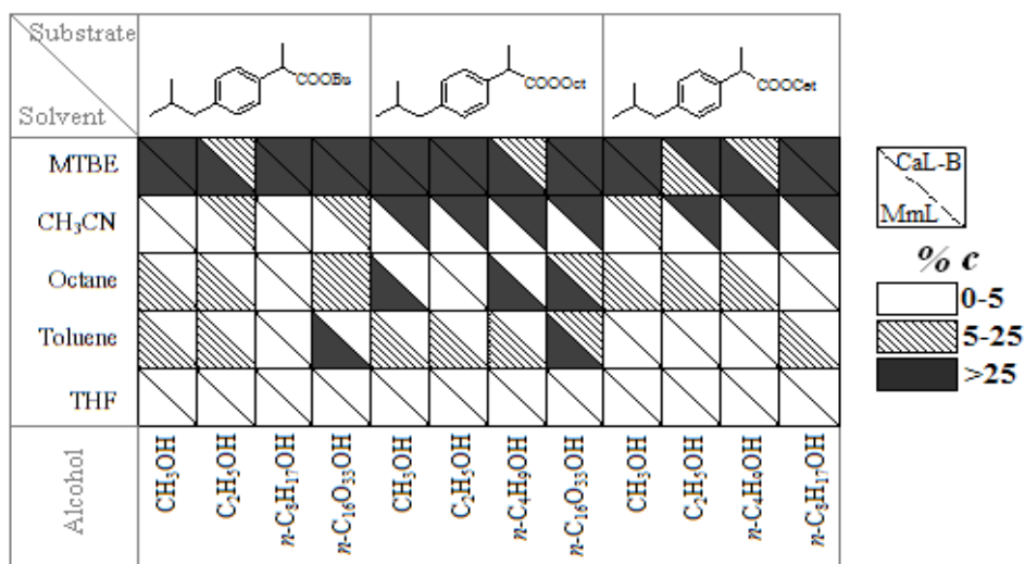
Figure 1. Conversions for the CaL-B and MmL mediated alcoholysis of rac-1c,d,e in various solvents at room temperature, after 17h
