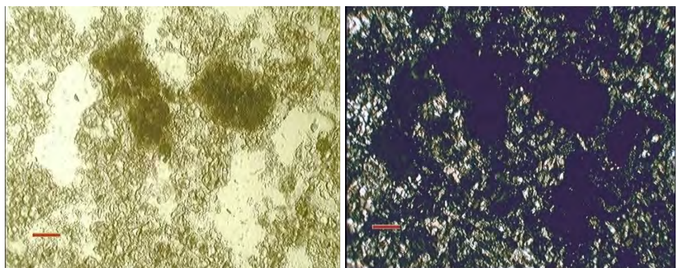
Figure 6. a (1N), b (N+). Sample 11B, fired at 1260°C: two drops of brownish olive interstitial material (isotropic sulphoaluminate in N+) between alitic (bottom left: polygonal grains) nests, belite I and belite III spherulites with rare alitic relics (dark grey birefringence). Scale bar 50 \mu\text{m}
