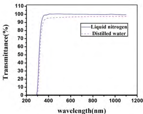
Figure 2. Optical transmittance spectra of the graphene nanosheets Produced in liquid nitrogen and distilled water environments
